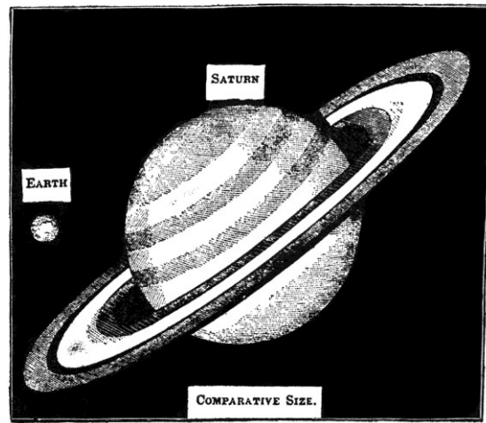
i060d2 Earth and Saturn Compared.
