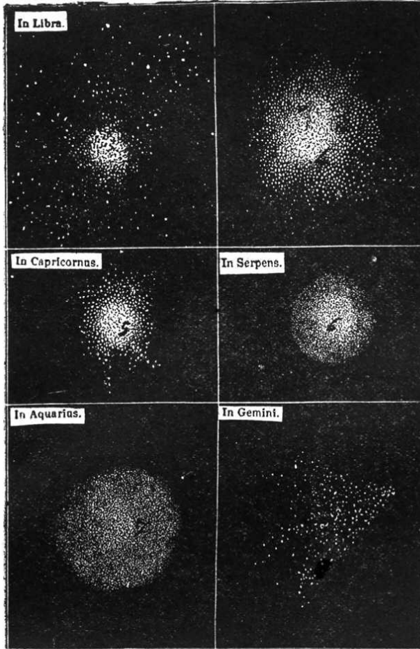
STAR CLUSTERS.
