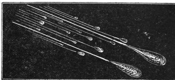
FIRE-BALL (as observed in a Telescope).
