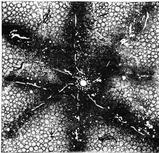
i010 The Earth in Jy'ay. The earth (white spot) in Jy'ay (ji'ay) during the glacial period, showing m'ha'k, the surrounding nebula, that caused
