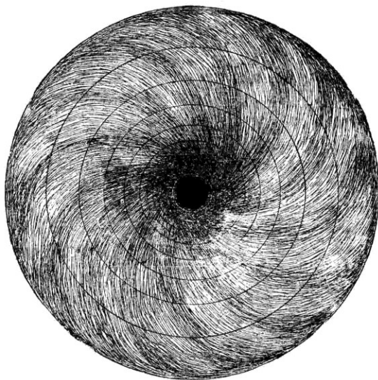
i005 Earth and Atmospherea , (as seen through spiritual eyes). Jehovih
