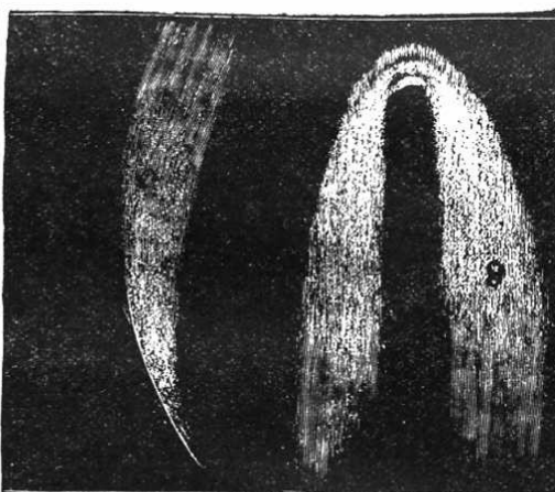
DONATI'S COMET. (General view.) DONATI'S COMET. (Showing the head and envelopes.)
